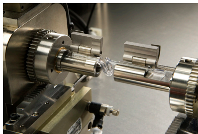
Tube Loop Forming Machine
